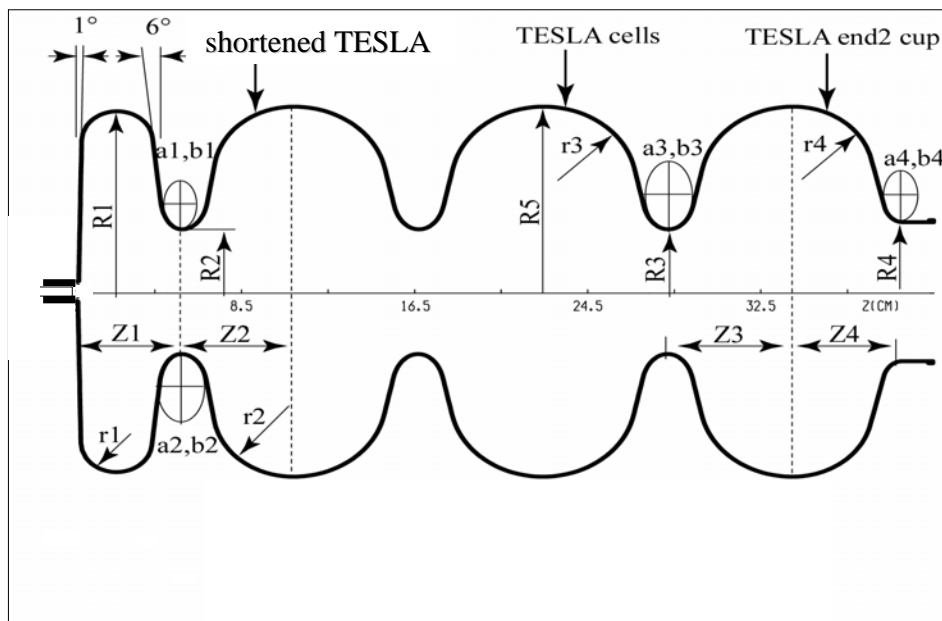
Fig. 1: Schematic cavity layout with design parameters.
